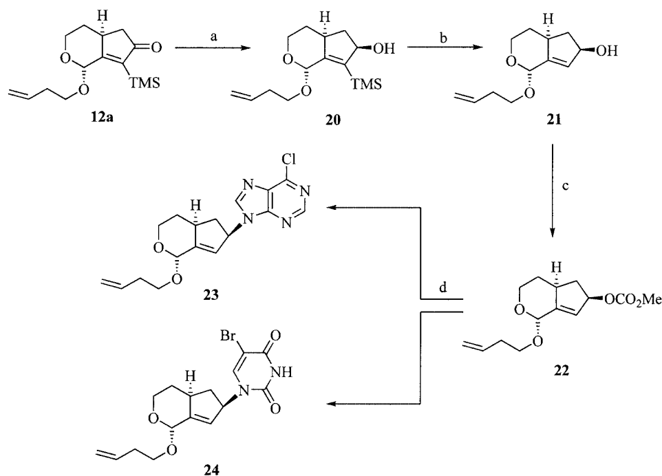
Scheme 5. Synthesis of the CNA precursors rac - 23 and rac - 24 . Reaction conditions: a) NaBH 4 (5 equiv.), CeCl 3 (1 equiv.), MeOH, –20 °C to room temp., 2 h, 99%; b) t BuOK (1 equiv.), DMSO/H 2 O (19:1), room temp., 2 h, 81%; c) ClCO 2 Me (3 equiv.), py, 0 °C, 1 h, 91%; d) [Pd 2 (dba) 3 ] (5 mol-%), dppp (10 mol-%), chloropurine or bromouracil (1.5 equiv.), DMF, room temp., 16 h, 60% for rac - 23 ; 73% for rac - 24 .
