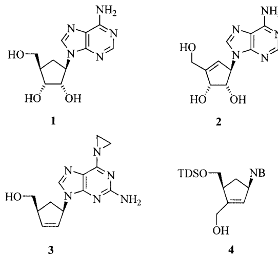
Scheme 1. Selected examples of CNAs (carbocyclic nucleoside analogs). NB = nucleobase.
