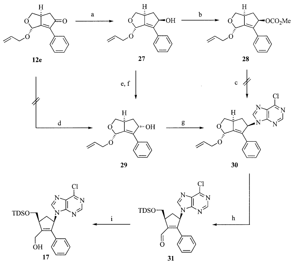
Scheme 7. Synthesis of the 2'-phenyl-substituted nucleoside analog rac - 17 . Reaction conditions: a) \text{NaBH}_4 (4 equiv.), \text{CeCl}_3 (1 equiv.), \text{MeOH} , -20^\circ\text{C} to room temp., 2 h, 99%; b) \text{ClCO}_2\text{Me} (3 equiv.), \text{py} , 0^\circ\text{C} , 1 h, 84%; c) [\text{Pd}_2(\text{dba})_3] (5 mol-%), \text{dppp} (10 mol-%), chloropurine (1.5 equiv.), \text{DMF} , room temp., 16 h; d) Yamamoto's reagent (from 2,6-di- tert -butyl-4-methylphenol and \text{DIBAL} ), [27a] toluene, -78^\circ\text{C} to -40^\circ\text{C} , 5 h; e) \text{DEAD} (5 equiv.), \text{PPh}_3 (5 equiv.), p -nitrobenzoic acid (4.4 equiv.), toluene, room temp., 16 h, 79%; f) \text{K}_2\text{CO}_3 (2 equiv.), \text{MeOH} , room temp., 16 h, 82%; g) \text{DEAD} (2 equiv.), \text{PPh}_3 (2 equiv.), chloropurine (2 equiv.), \text{THF} , room temp., 16 h, 62%; h) \text{PPTS} (0.3 equiv.), wet acetone, reflux, 6 h; then \text{TDSCl} (4 equiv.), \text{py} , room temp., 16 h, 73% over 2 steps; i) \text{NaBH}_4 (10 equiv.), \text{MeOH}/\text{CH}_2\text{Cl}_2 , -78^\circ\text{C} , 1 h, 99%.
