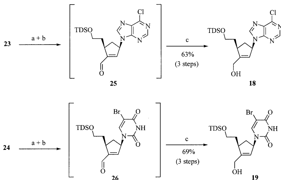
Scheme 6. Preparation of the CNAs rac - 18 and rac - 19 . Reaction conditions: a) Amberlyst-15 (0.1 wt. equiv.), wet acetone, room temp., 1 h, then poly(4-vinylpyridine) (2 wt. equiv.); b) TDSOCl (3 equiv.), py, room temp., 16 h; c) NaBH 4 (10 equiv.), MeOH/CH 2 Cl 2 , –78 °C, 1 h.
