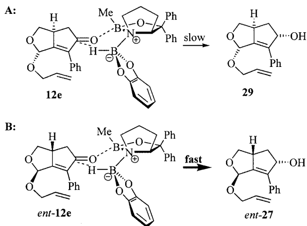
Scheme 9. Two competing transition structures for the kinetic resolution of rac - 12e by CBS reduction assuming catalyst control. A: mismatched case (violation of substrate preference); B: matched case.
