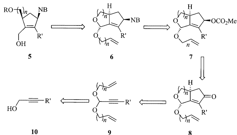
Scheme 2. Retrosynthetic analysis for CNAs of type 5 .
