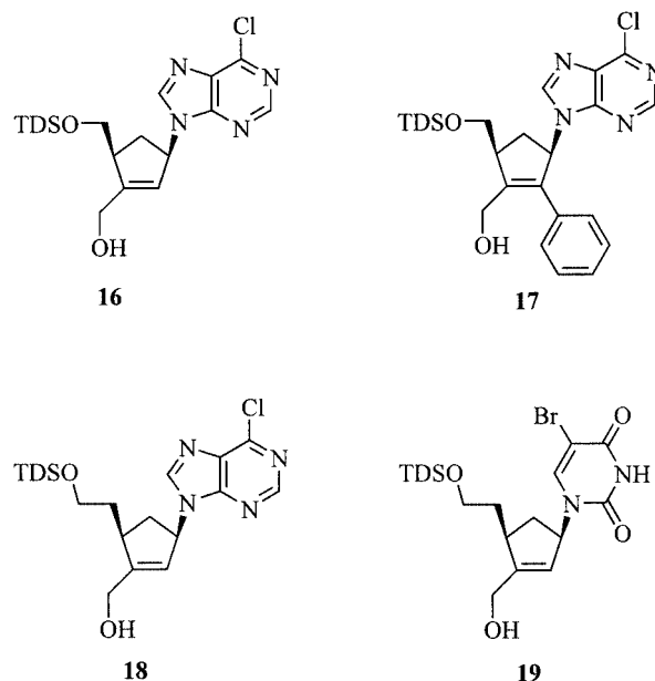
Scheme 4. The apoptosis-inducing CNA 16 [10a] and the envisioned structural analogs 17–19 (as target structures).
