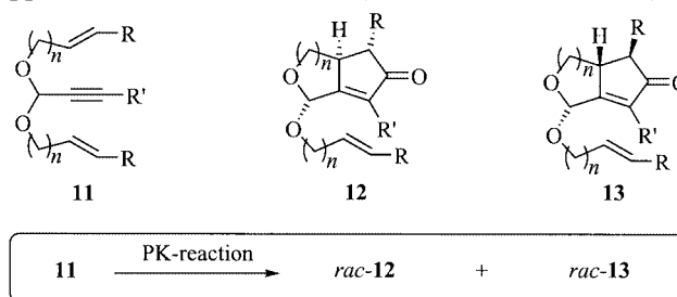
Scheme 3. General pattern of the Pauson–Khand reactions investigated (see Table 1 for yields and diastereoselectivities).
